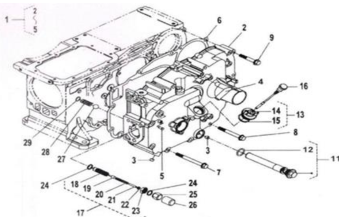
CASE GEAR COMP.
