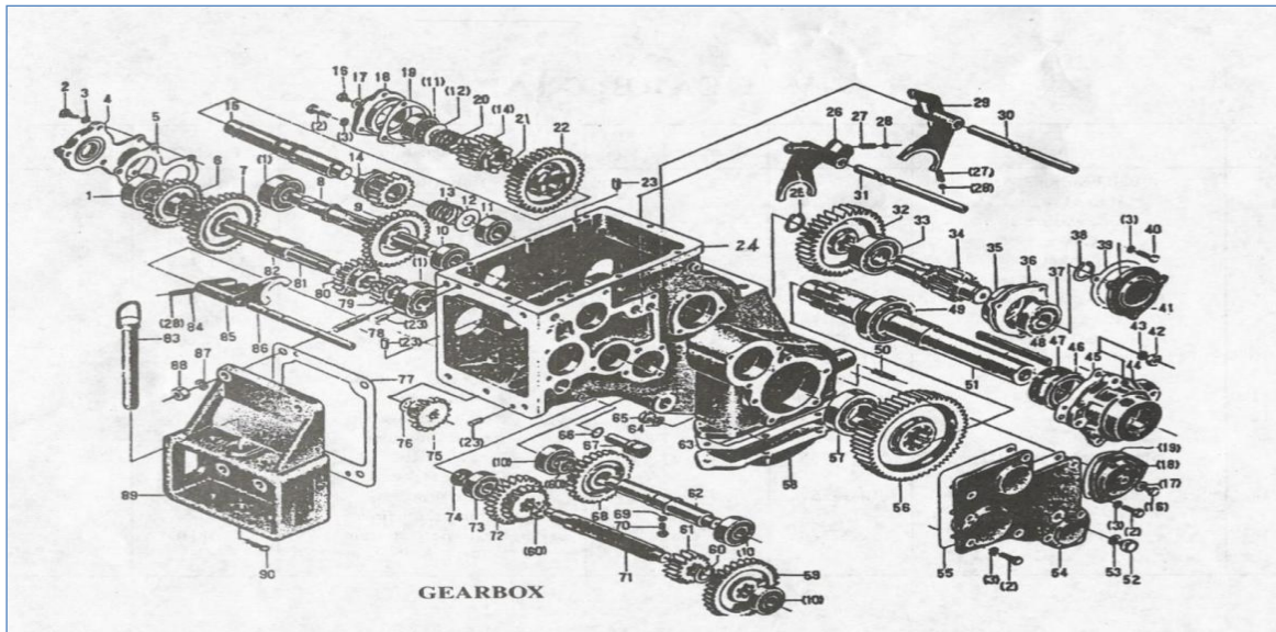
Gear Box (A) (Fig. IV)
