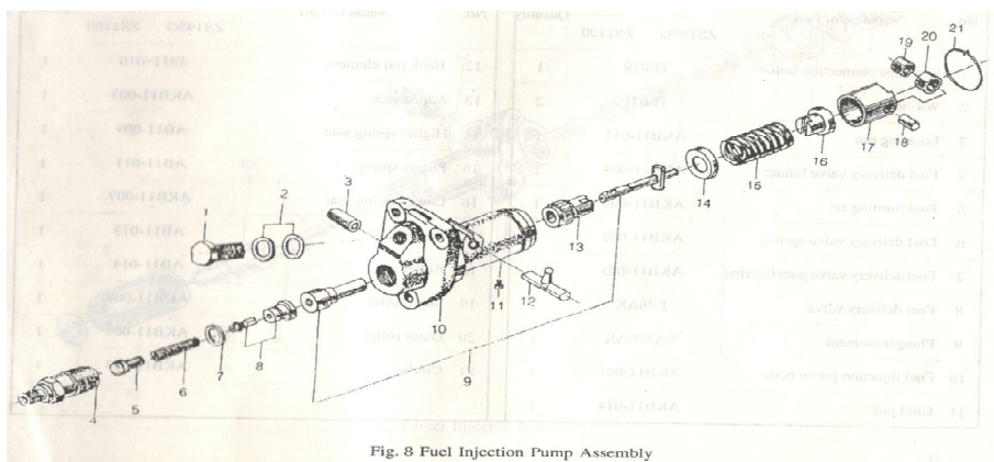
Fig. 8 Fuel Injection Pump Assembly
