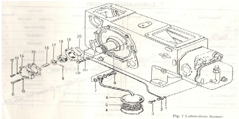
Fig. 7 Lubrication System
