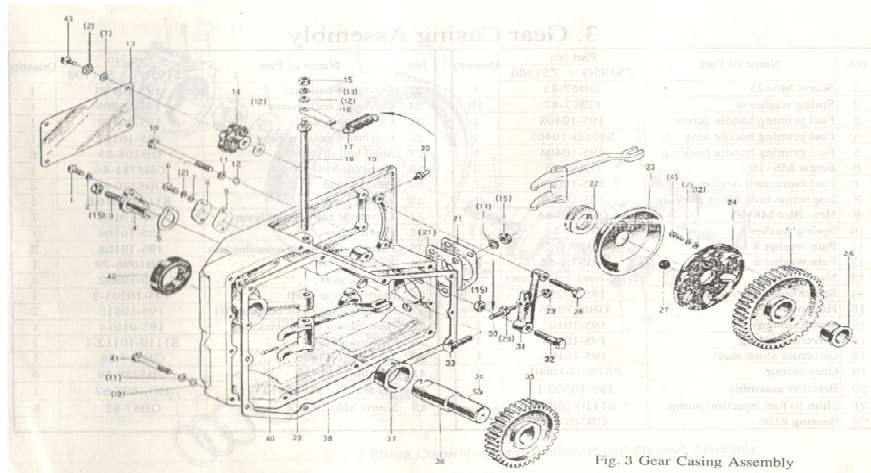
Fig. 3 Gear Casing Assembly
